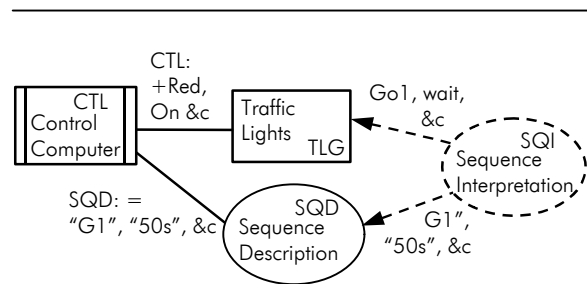
Figure 6 Flexible Traffic Lights Problem
