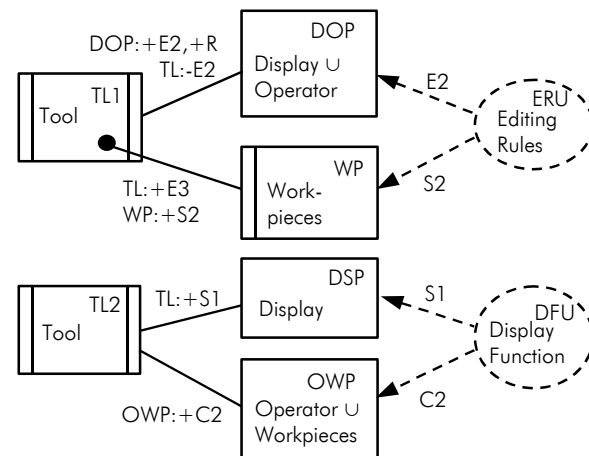
Figure 12 Decomposition of Visible Workpieces Frame
