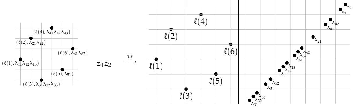
Figure 2: The mapping \Psi : \mathcal{C} \wr (\mathbb{L} \times \mathbb{L}^*) \times \mathbb{L}^* \rightarrow \mathcal{C} \wr \mathcal{D} \wr \mathbb{L} .
